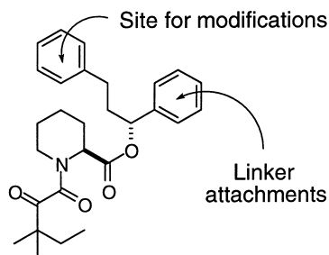
Figure 2. Prototypical synthetic ligand used as basis for synthetic CIDs.
