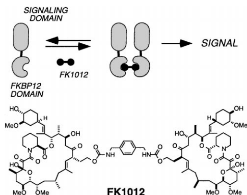
Figure 1. FK1012, a chemical inducer of dimerization (CID).
