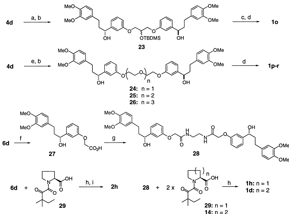
Scheme 3. Reagents and conditions: (a) i. epibromohydrin, KO t -Bu, DMF, 100 °C; ii. TBDMS-Cl, imidazole, DMF, 0 °C; (b) (+)-DIP-Cloride®, THF, -20 °C; (c) 2 equiv 14 , DCC, DMAP, CH 2 Cl 2 , 0 °C; (d) 49% HF, CH 3 CN. (e) diiodide, NaH, DMF; (f) 6 N NaOH, MeOH; (g) ethylenediamine, PyBOP, THF, TEA, 0 °C; (h) DCC, DMAP, CH 2 Cl 2 , 0 °C; (i) TFA, CH 2 Cl 2 , 0 °C.
