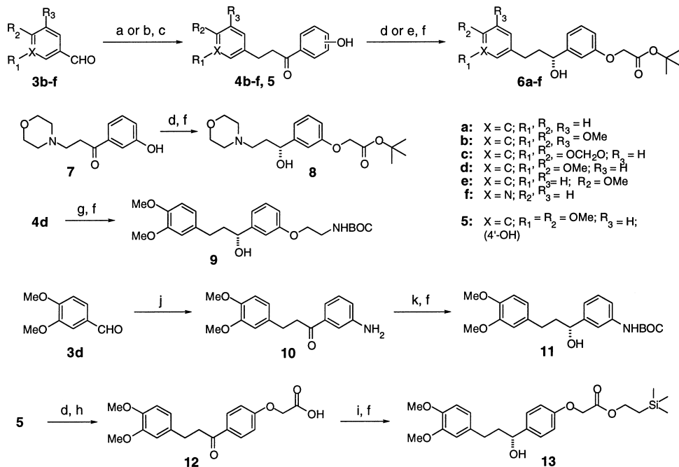
Scheme 1. Reagents and conditions: (a) 3'-Hydroxyacetophenone or 4'-hydroxyacetophenone, KOH, H 2 O/EtOH, 0 °C; (b) 3'-hydroxyacetophenone, piperidine, reflux; (c) H 2 , Lindlar catalyst, MeOH; (d) tert -butyl bromoacetate, K 2 CO 3 , DMF, 0 °C; (f) (+)-DIP-Chloride ® , THF, -20 °C; (g) BrCH 2 CH 2 NHBOC, NaI, K 2 CO 3 , DMF, 60 °C; (h) TFA, CH 2 Cl 2 , 0 °C; (i). TMSCH 2 CH 2 OH, DCC, DMAP, CH 2 Cl 2 , 0 °C; (j) i. 3'-nitroacetophenone, KOH, H 2 O/EtOH, 0 °C; ii. H 2 , Lindlar catalyst, MeOH; (k) (BOC) 2 O, DIEA, CH 2 Cl 2 .
