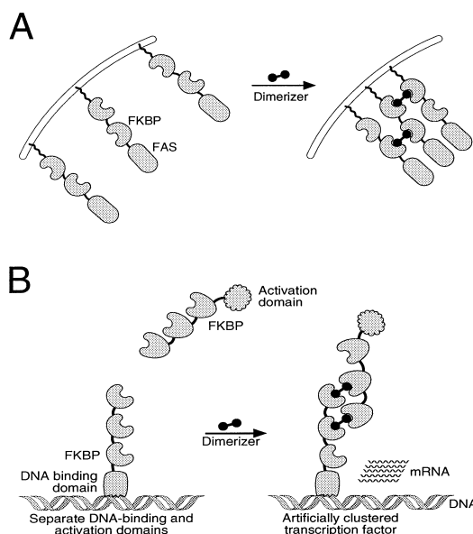
Figure 3. Schemes for obtaining dimerizer-dependent (A) apoptosis via Fas activation; and (B) regulation of gene expression.
